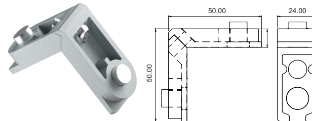
QV221 10X24MM ADJUSTABLE CORNER CLEAT
