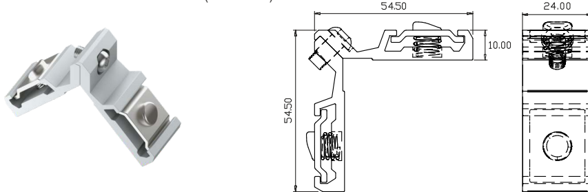
QV204 10X24MM ADJUSTABLE CORNER CLEAT (PREMIUM)
