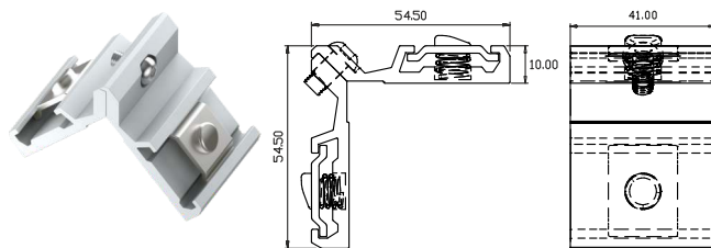
QV211 10X41MM ADJUSTABLE CORNER CLEAT (PREMIUM)
