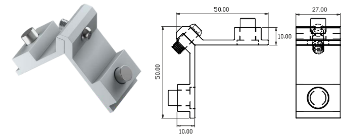
QV206 10X27MM ADJUSTABLE CORNER CLEAT
